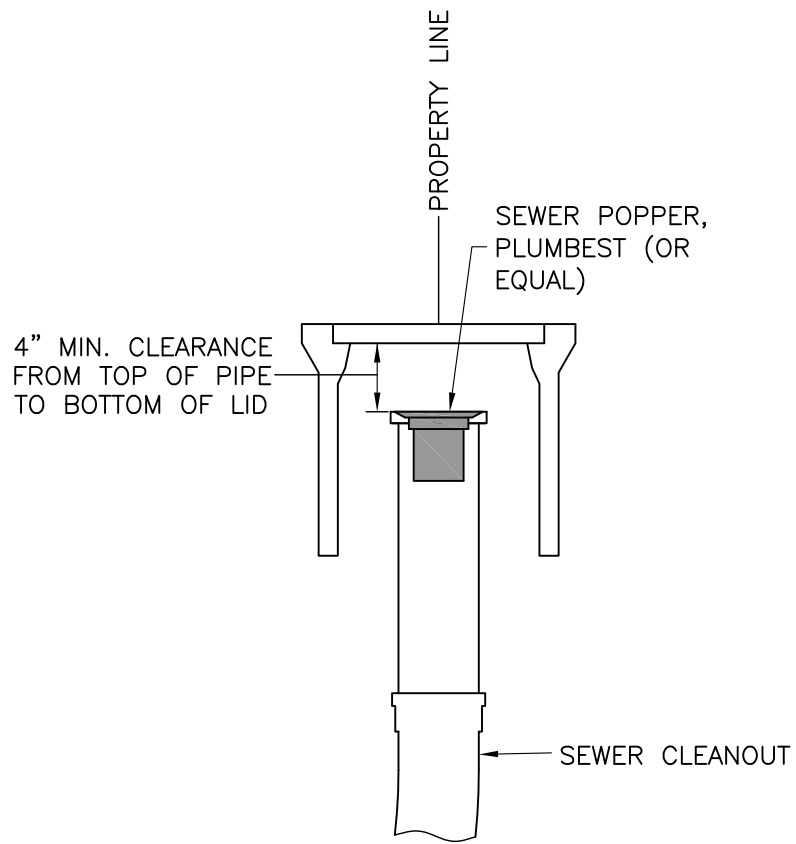
POPPER ON CLEANOUT
